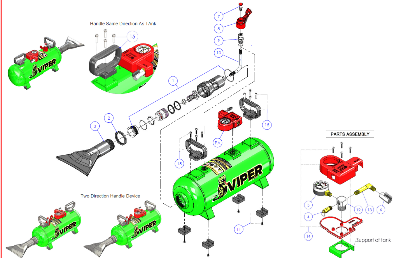
VP-18AL GEN 3.0 Main Assembly
