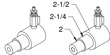
Extra Large Step Adapters
